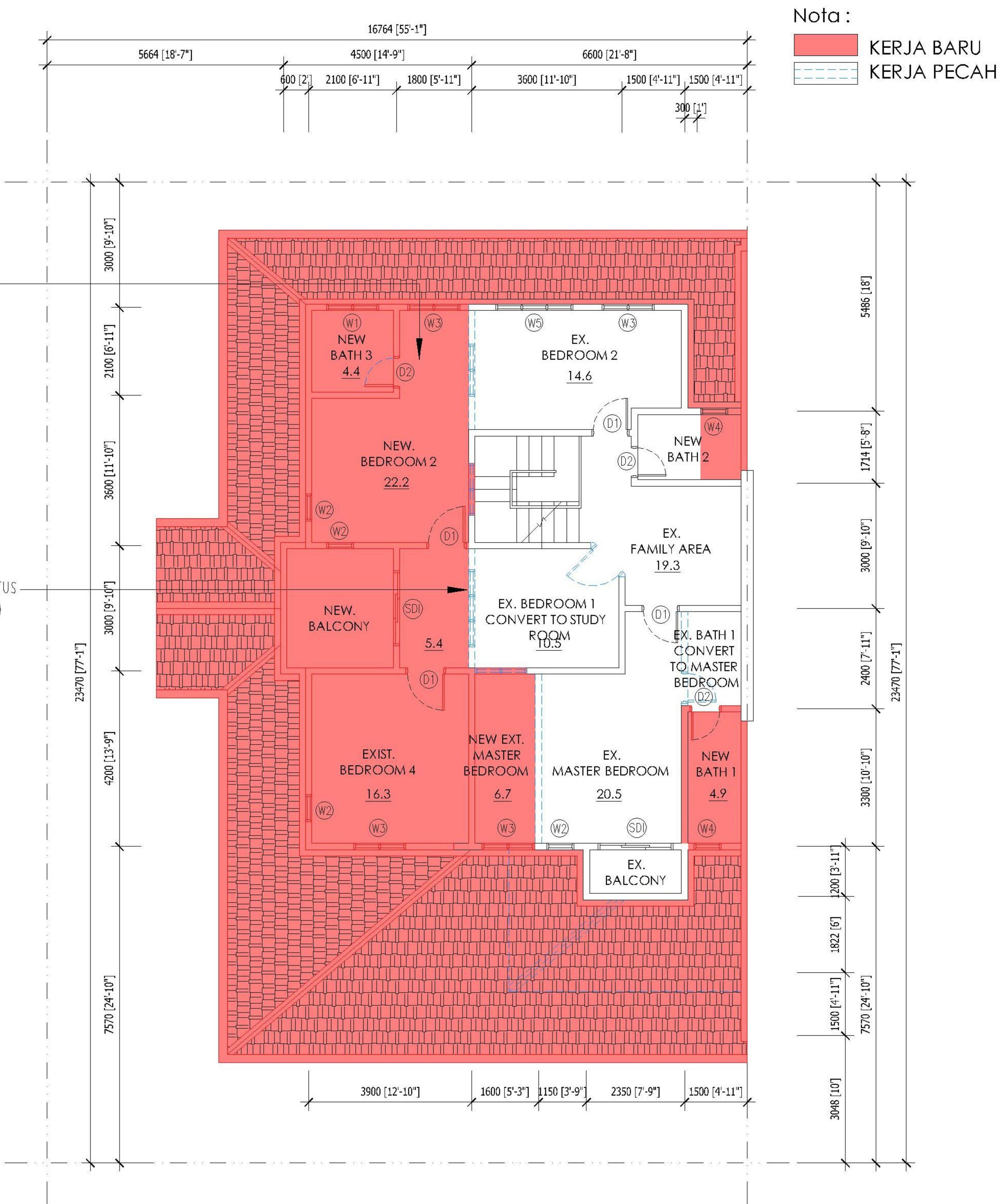
First Floor Plan scale 1:100
